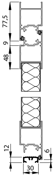
DoorPro 45, Profile Dimensions
